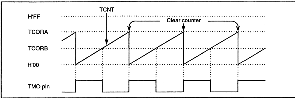
Figure 7-12. Example of Pulse Output
