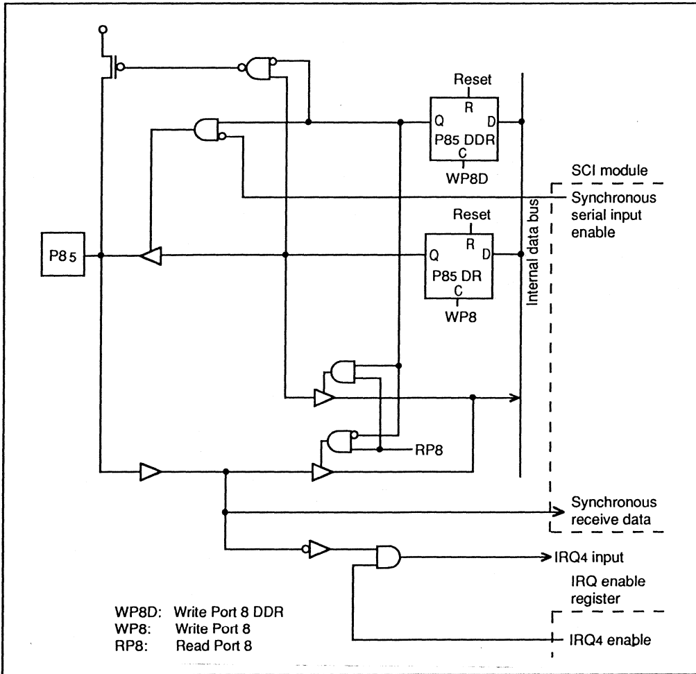
Figure 5-18. Port 8 Schematic Diagram (Pin P85)
