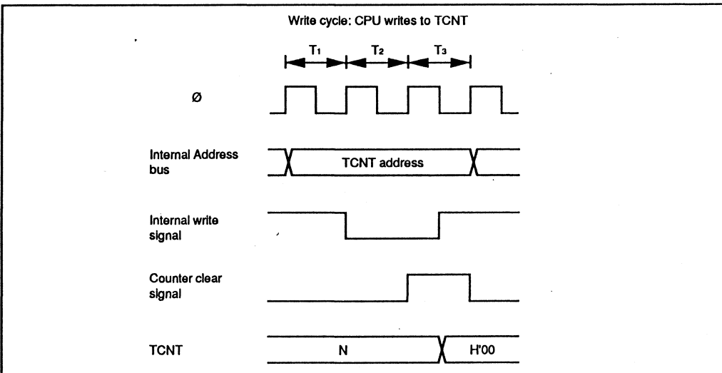
Figure 7-13. TCNT Write-Clear Contention
