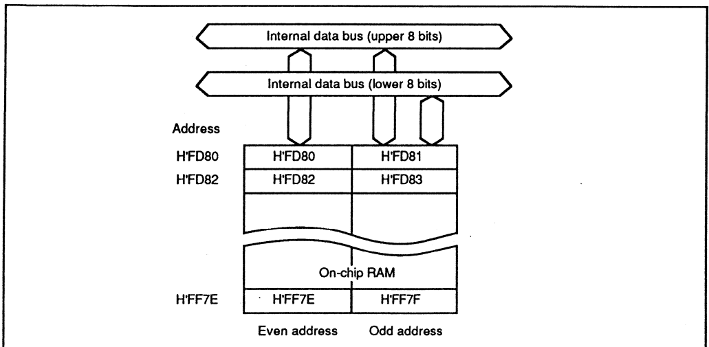
Figure 12-1. Block Diagram of On-Chip RAM
