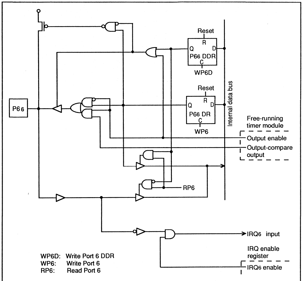
Figure 5-11. Port 6 Schematic Diagram (Pin P66)
