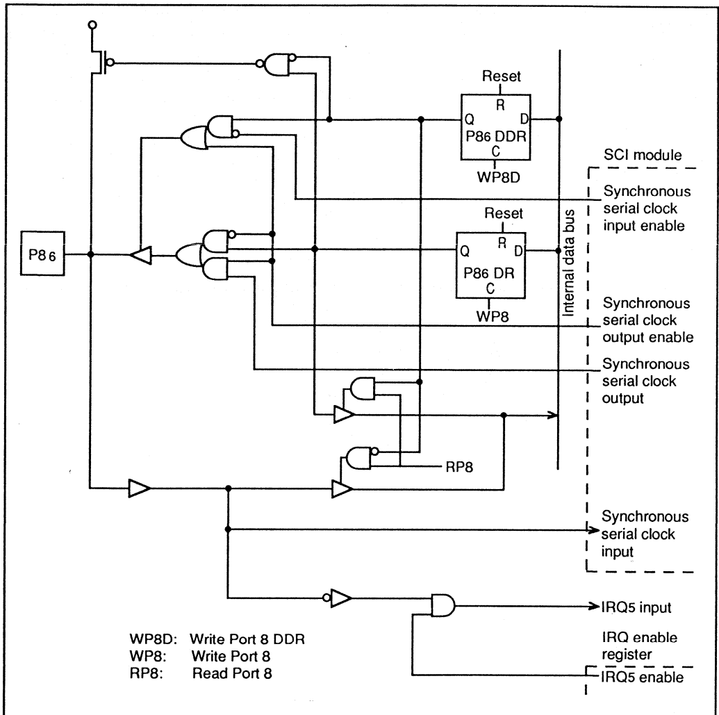
Figure 5-19. Port 8 Schematic Diagram (Pin P86)
