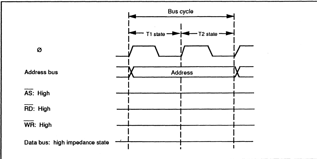
Figure 3-14. Pin States during On-Chip Memory Access Cycle
