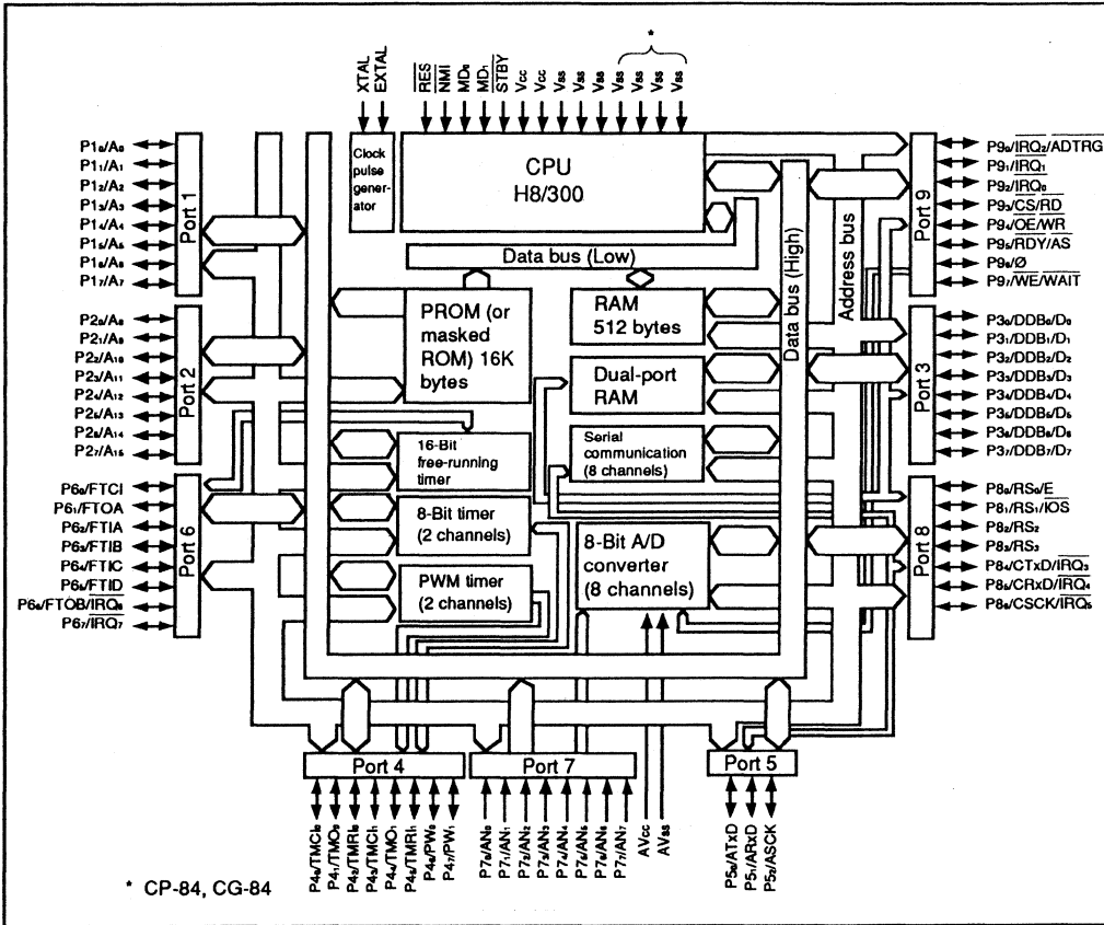
Figure 1-1. Block Diagram
