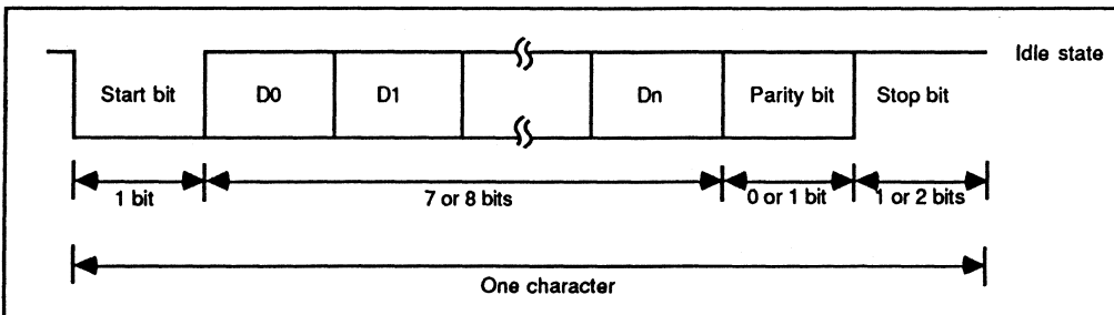
Figure 9-2. Data Format in Asynchronous Mode
