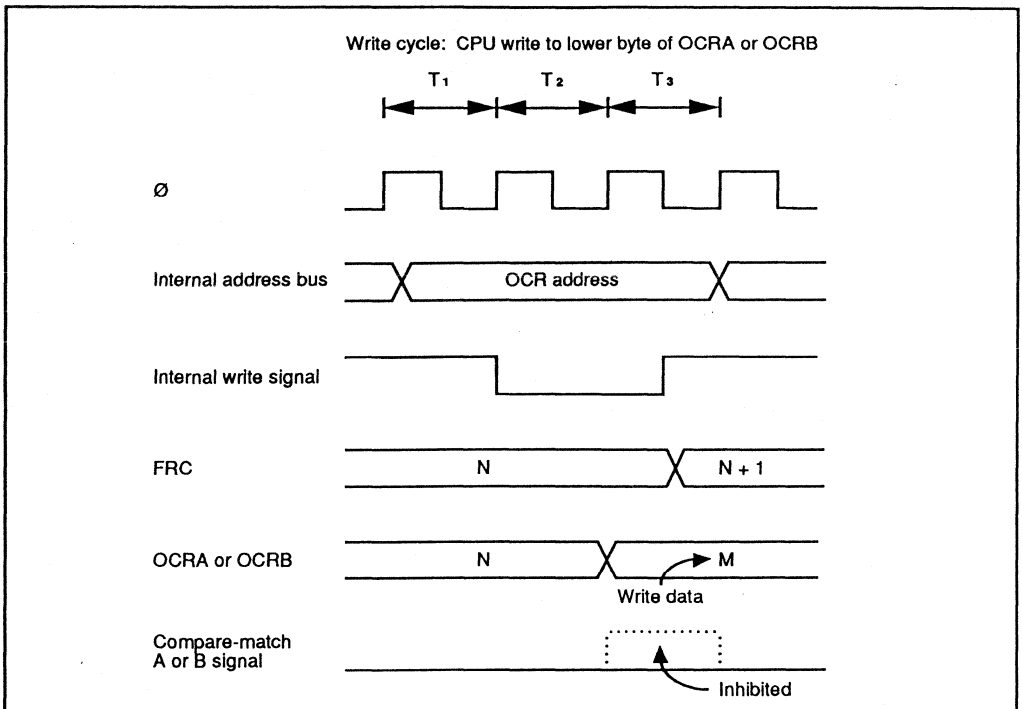
Figure 6-23. Contention between OCR Write and Compare-Match
