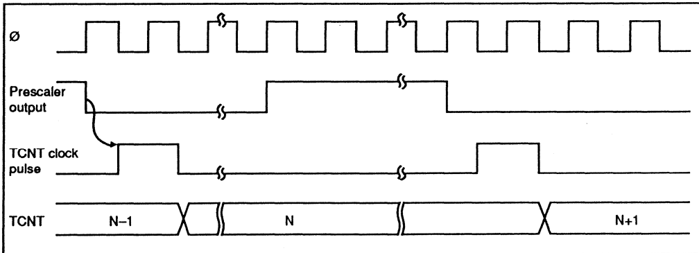
Figure 7-2. Count Timing for Internal Clock Input
