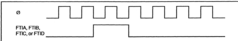
Figure 6-3. Minimum Input Capture Pulse Width
