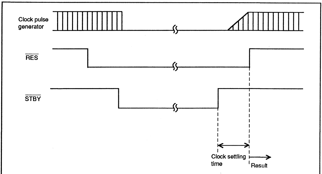
Figure 14-2. Hardware Standby Mode Timing
