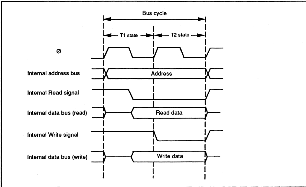
Figure 3-13. On-Chip Memory Access Cycle
