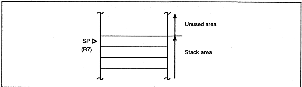
Figure 3-2. Stack Pointer
