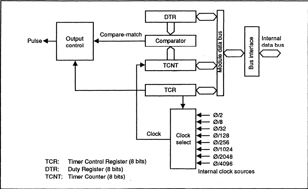
Figure 8-1. Block Diagram of PWM Timer
