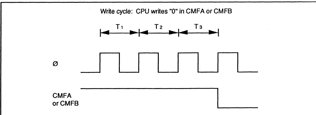
Figure 7-6. Clearing of Compare-Match Flags
