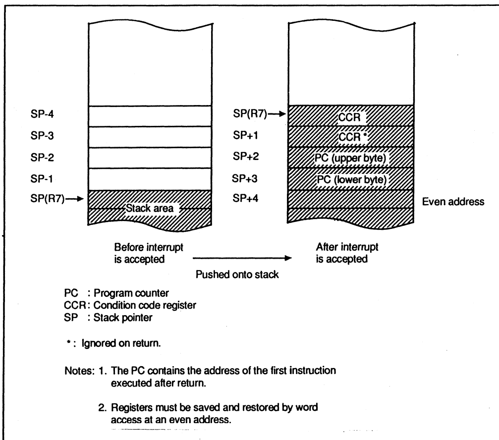
Figure 4-6. Usage of Stack in Interrupt Handling
