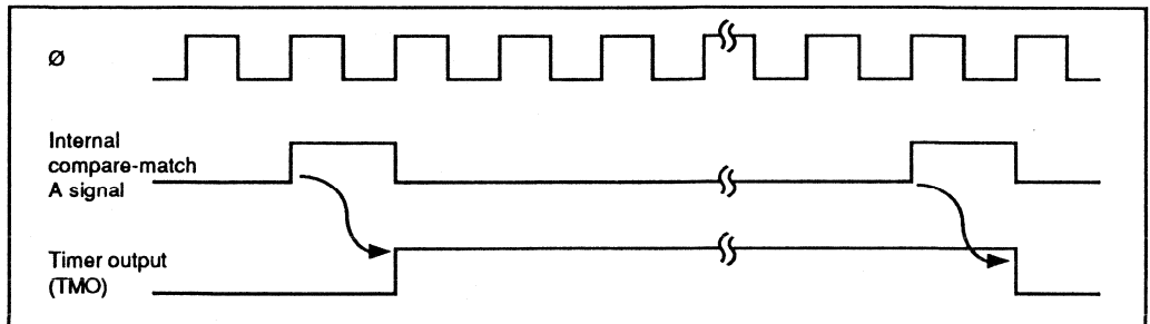
Figure 7-7. Timing of Timer Output
