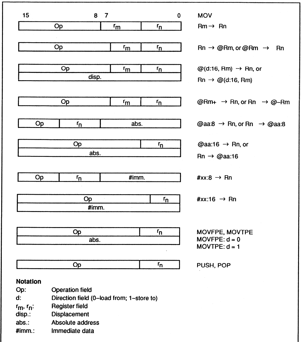
Figure 3-5. Data Transfer Instruction Codes
