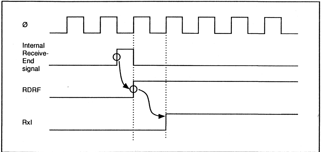
Figure 9-5. Timing of Interrupt Signal
