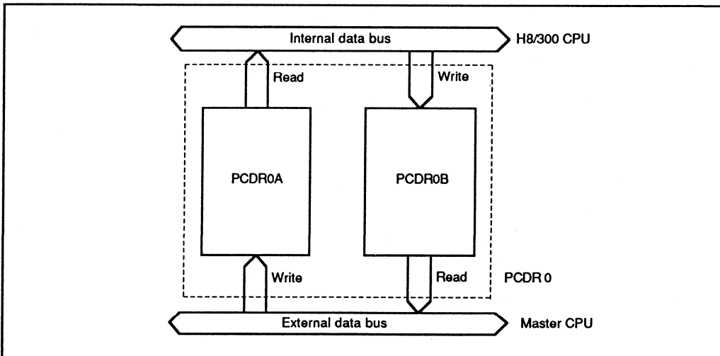
Figure 11-2. Parallel Communication Data Register 0
