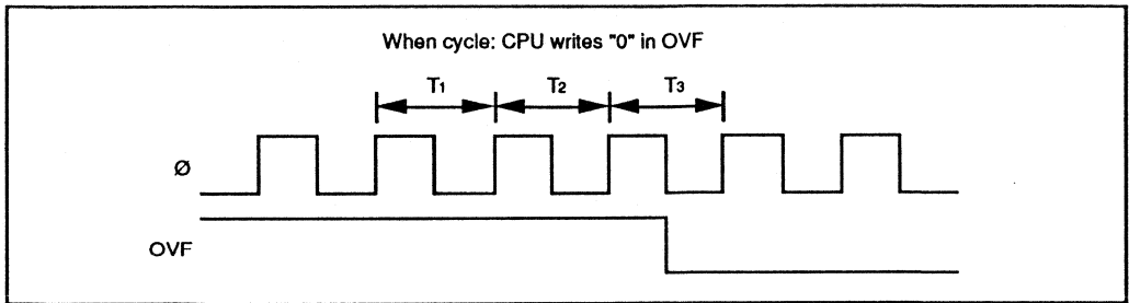
Figure 7-11. Clearing of Overflow Flag
