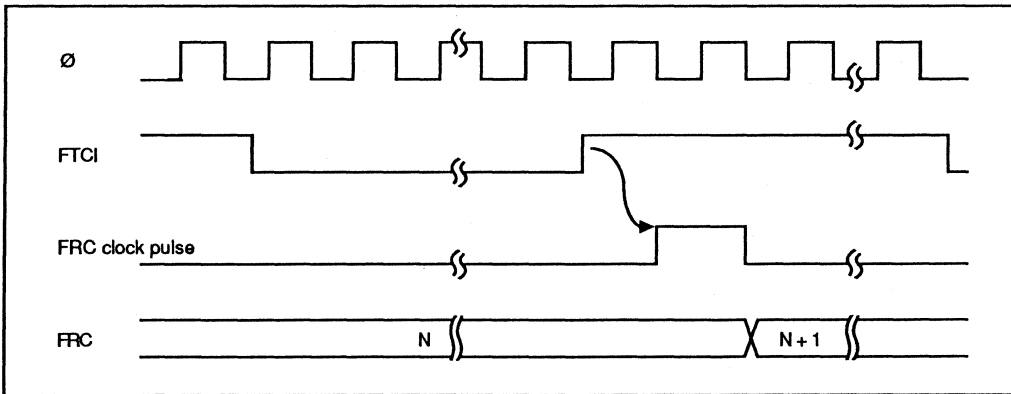
Figure 6-6. Increment Timing for External Clock Source
