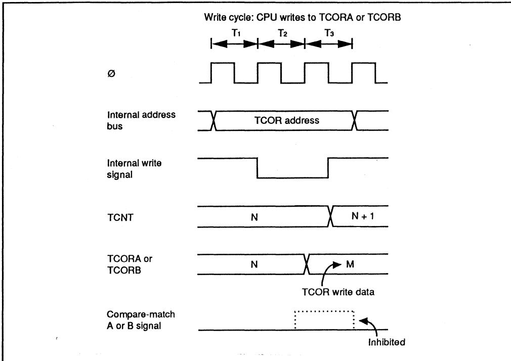
Figure 7-15. Contention between TCOR Write and Compare-Match
