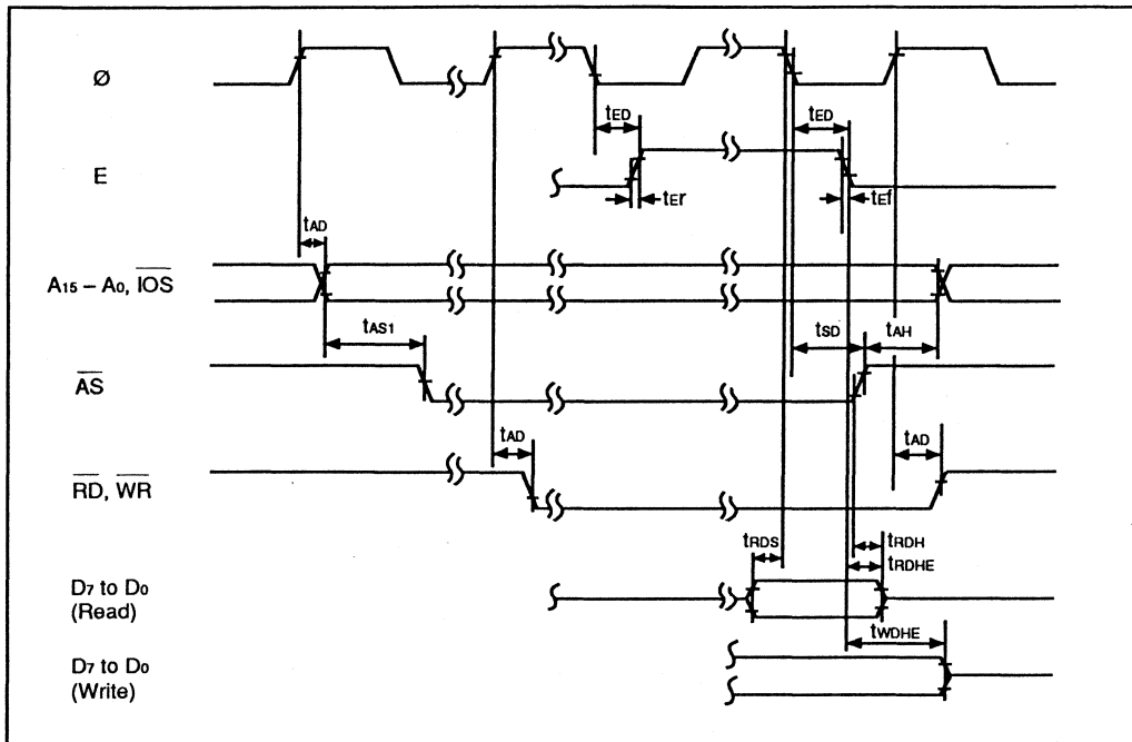
Figure 17-6. E Clock Bus Cycle
