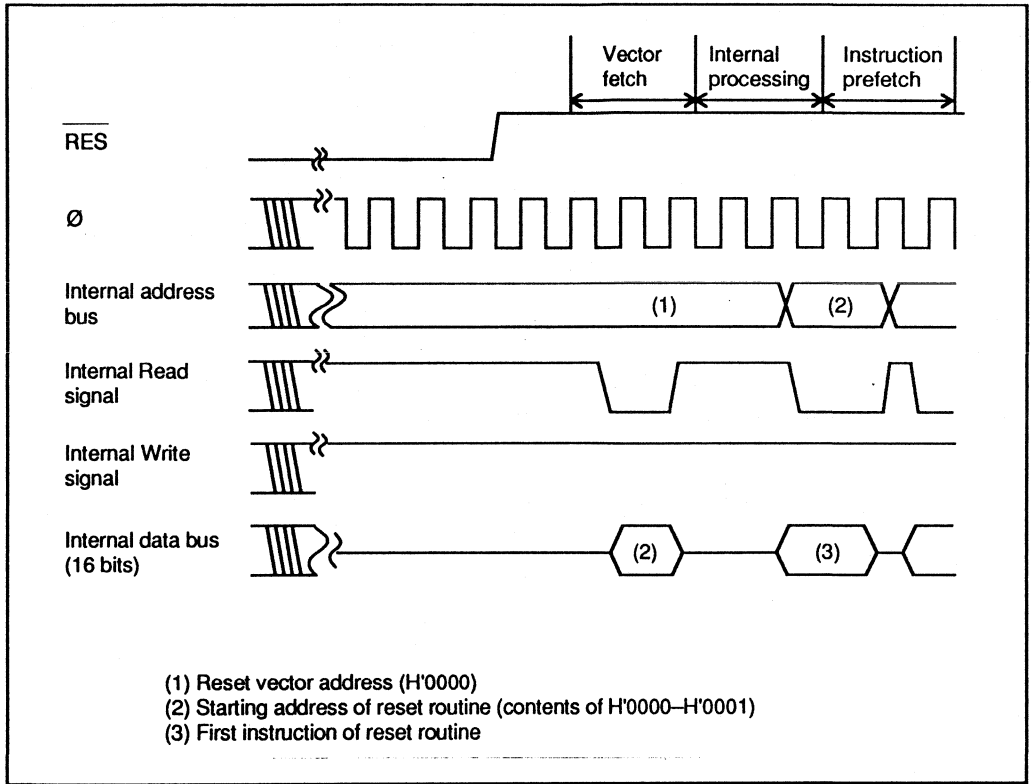
Figure 4-1. Reset Sequence (Mode 2 or 3, Reset Routine in On-Chip ROM)
