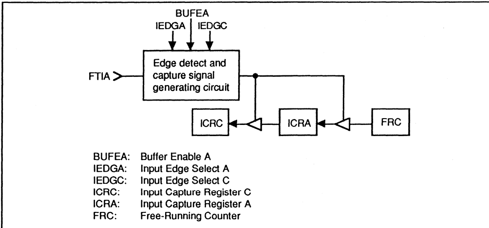
Figure 6-2. Input Capture Buffering
