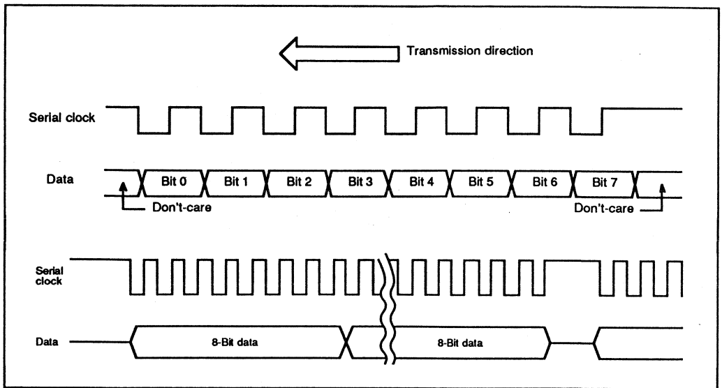
Figure 9-4. Data Format in Synchronous Mode
