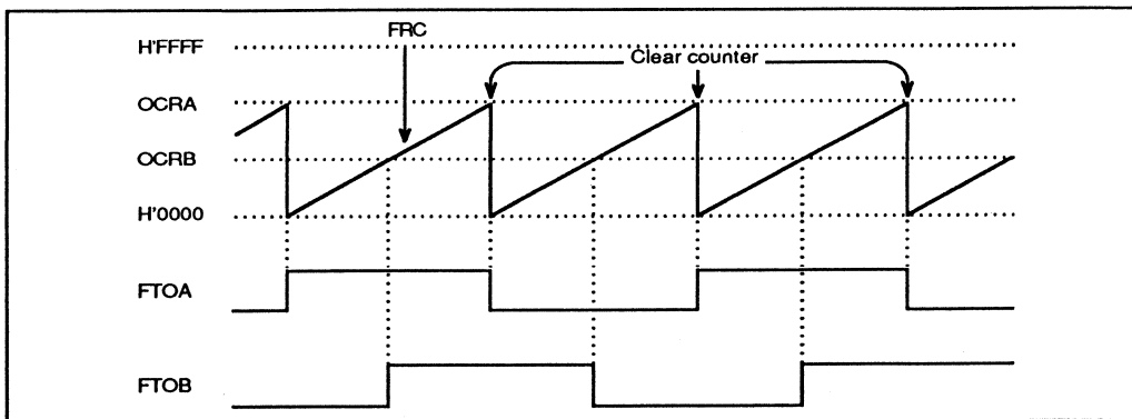
Figure 6-20. Square-Wave Output (Example)
