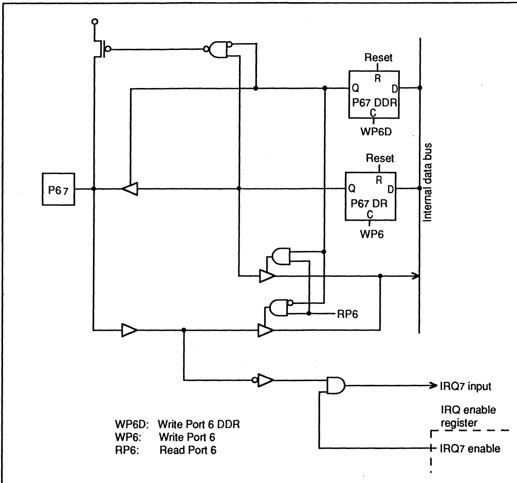
Figure 5-12. Port 6 Schematic Diagram (Pin P67)
