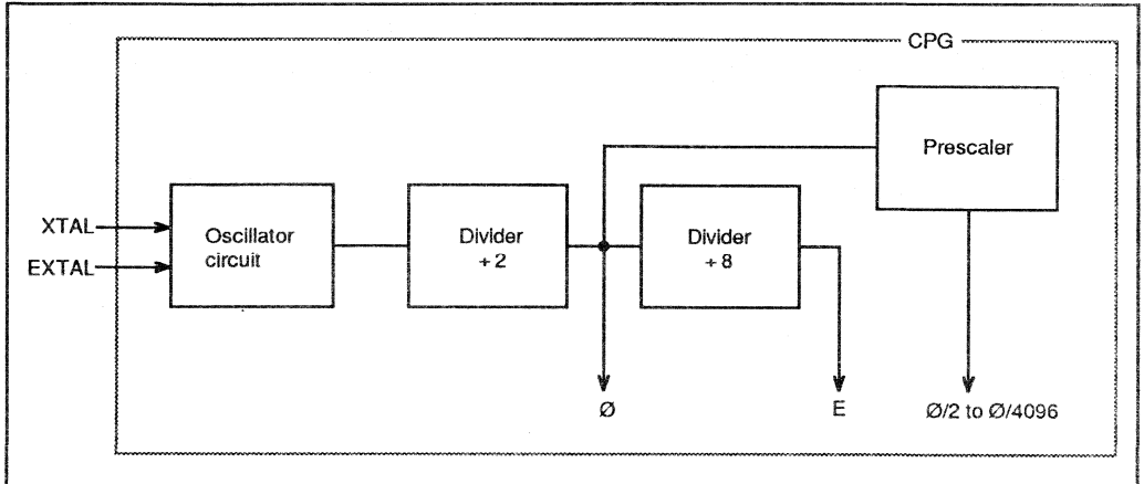
Figure 16-1. Block Diagram of Clock Pulse Generator
