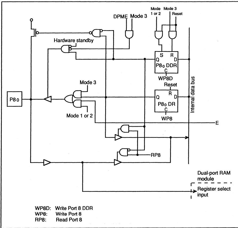
Figure 5-14. Port 8 Schematic Diagram (Pin P80)
