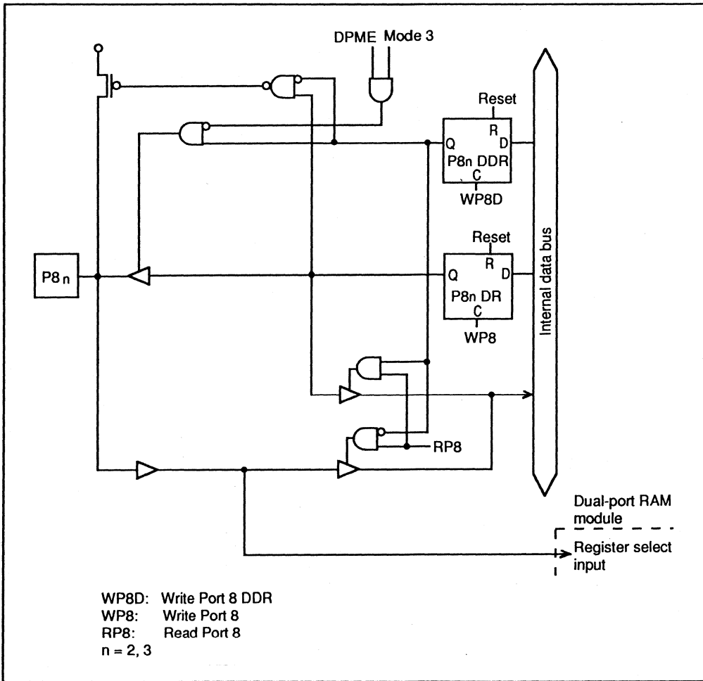
Figure 5-16. Port 8 Schematic Diagram (Pins P82 and P83)
