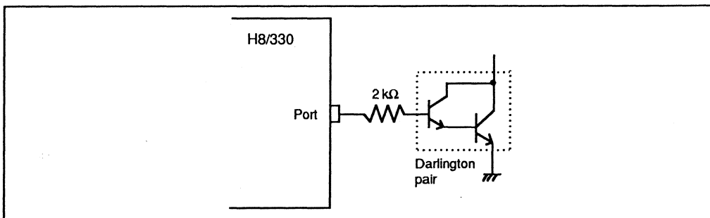
Figure 17-1. Example of Circuit for Driving a Darlington Pair
