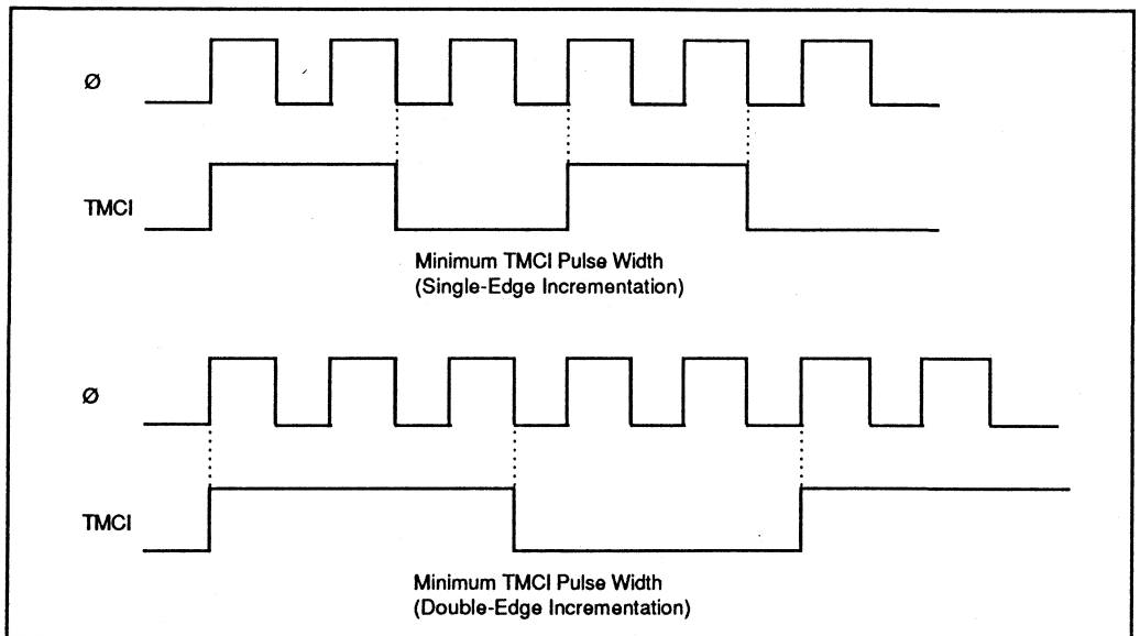
Figure 7-4. Minimum External Clock Pulse Widths (Example)
