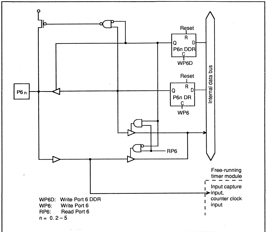
Figure 5-9. Port 6 Schematic Diagram (Pins P60, P62, P63, P64, and P65)
