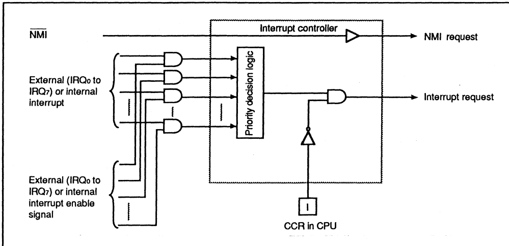
Figure 4-3. Block Diagram of Interrupt Controller
