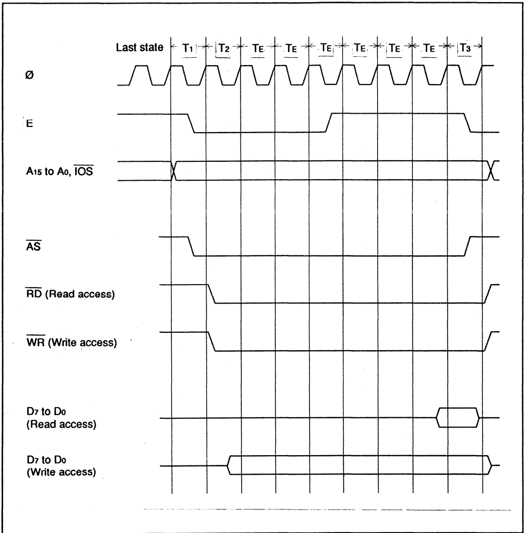
Figure 15-2. Execution Cycle of Instruction Synchronized with E Clock in Expanded Modes (Minimum Synchronization Delay)
