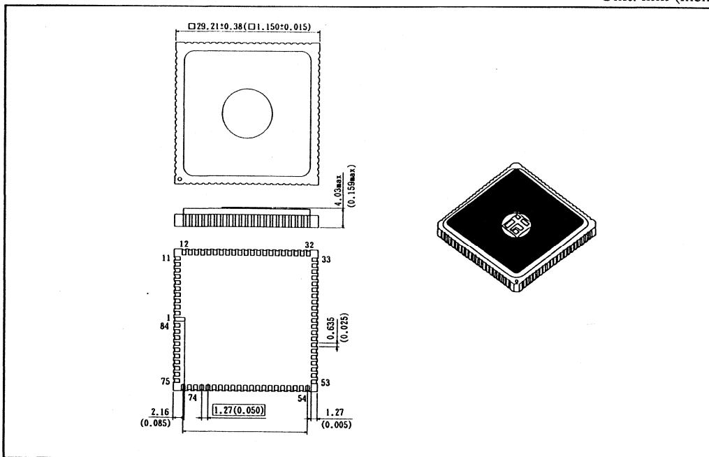
Figure D-1. Package Dimensions (CG-84)
