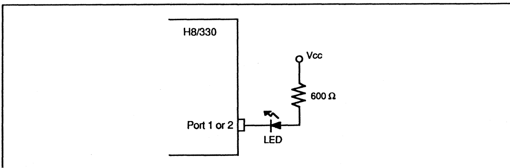
Figure 17-2. Example of Circuit for Driving a LED
