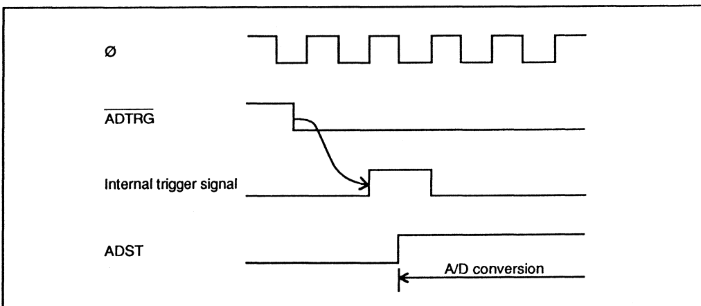
Figure 10-6. External Trigger Input Timing
