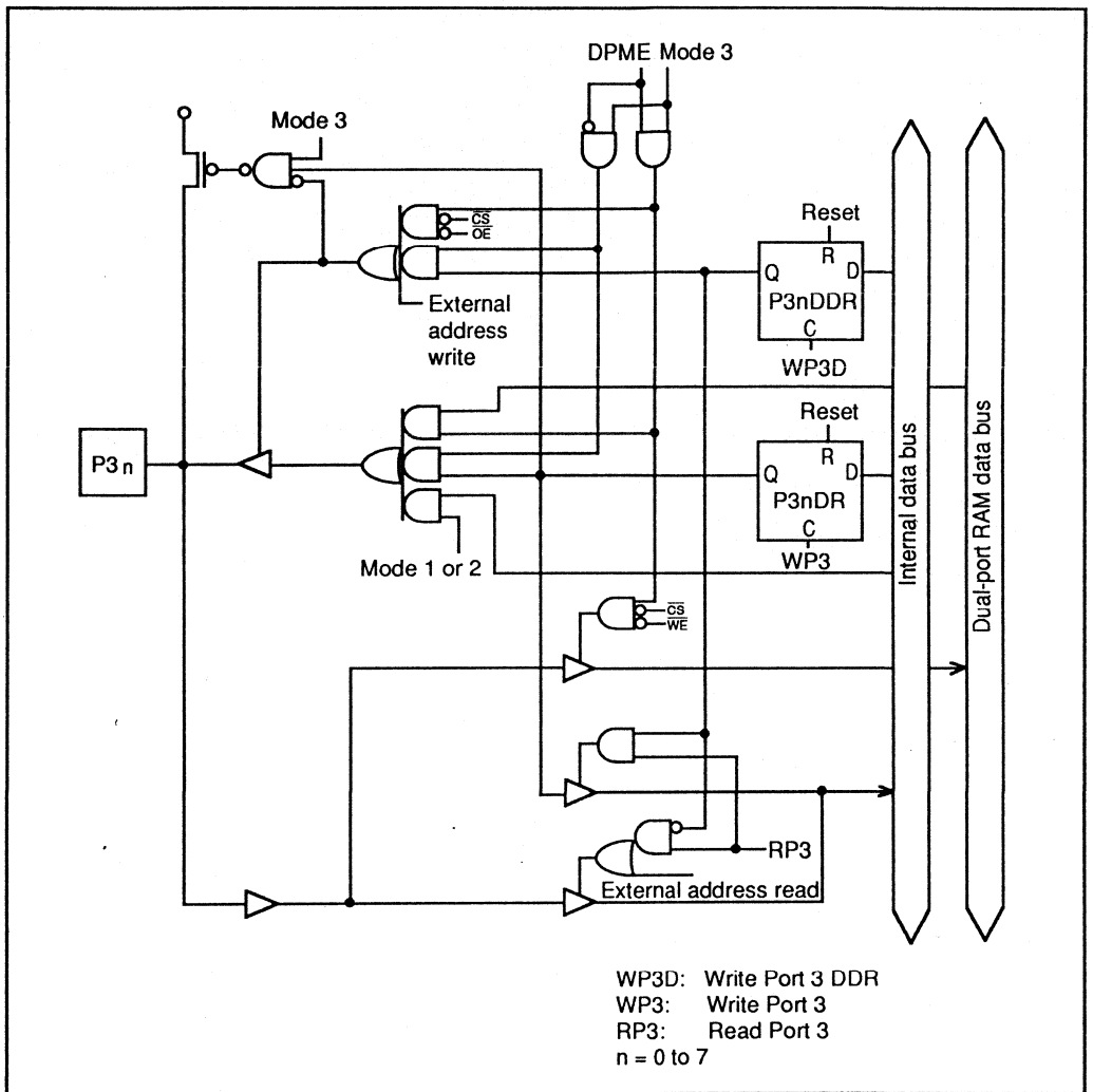
Figure 5-3. Port 3 Schematic Diagram
