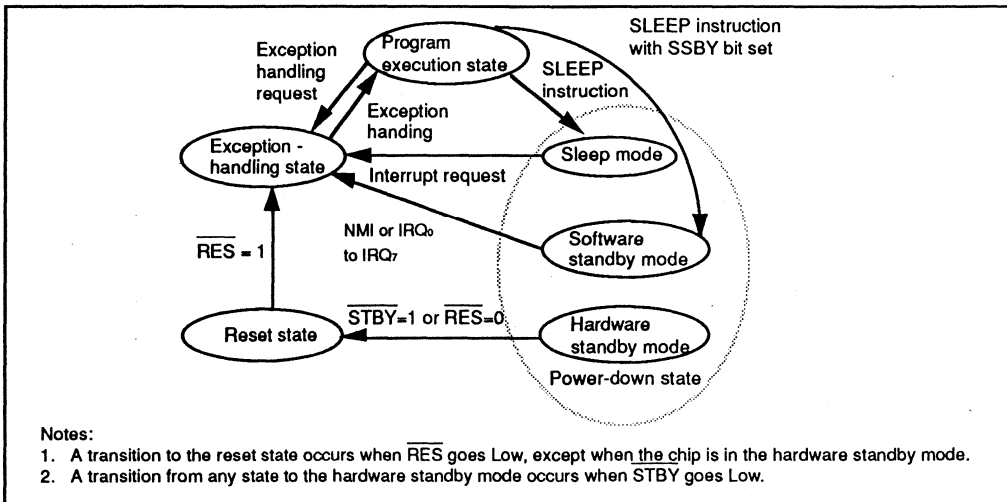
Figure 3-12. State Transitions
