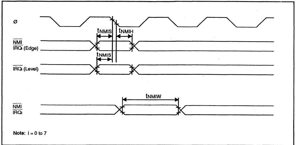
Figure 17-8. Interrupt Input Timing
