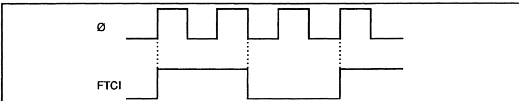
Figure 6-7. Minimum External Clock Pulse Width
