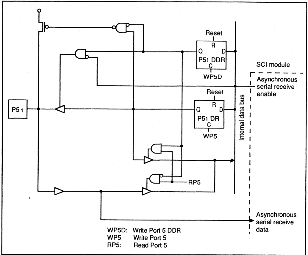
Figure 5-7. Port 5 Schematic Diagram (Pin P51)
