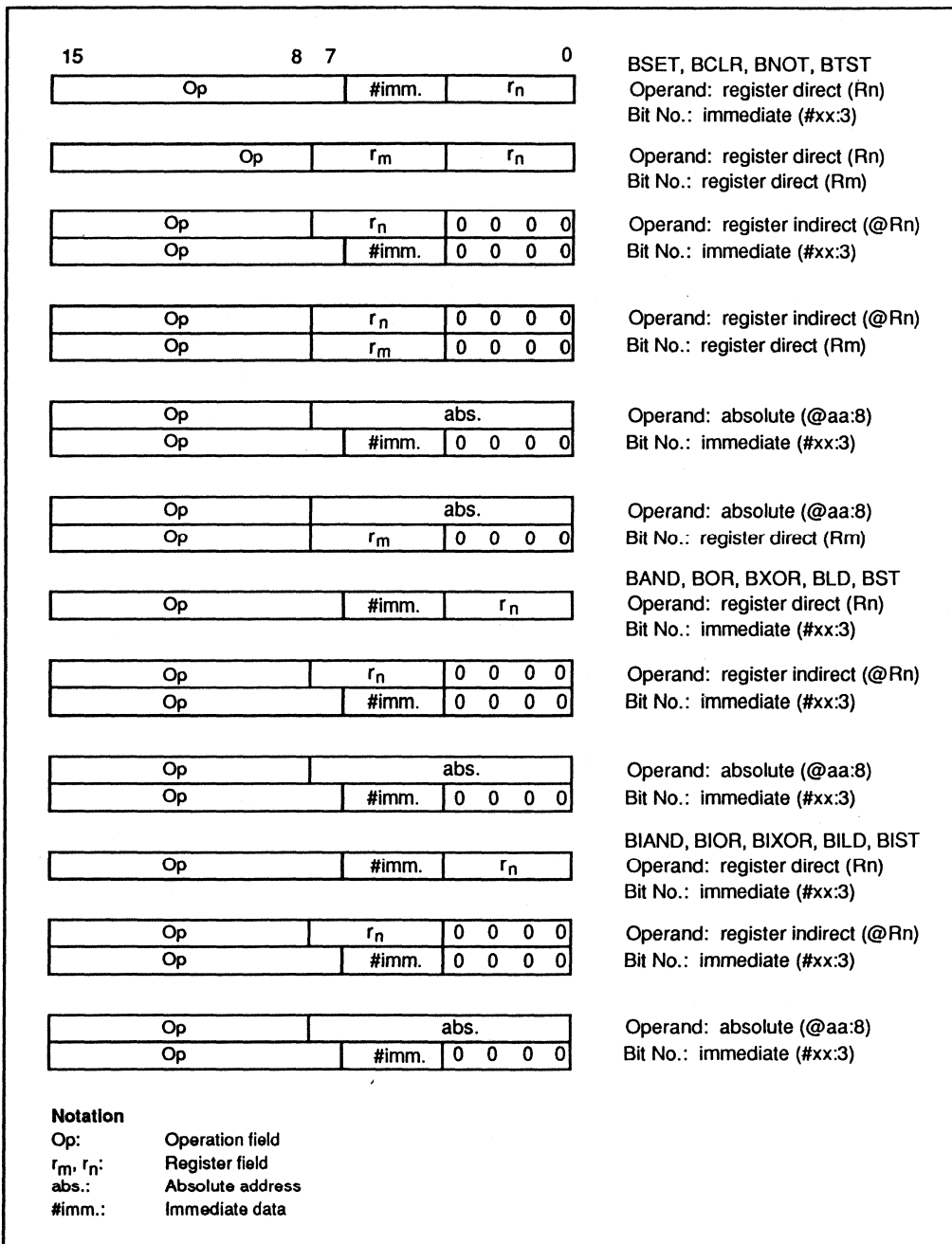
Figure 3-7. Bit Manipulation Instruction Codes
