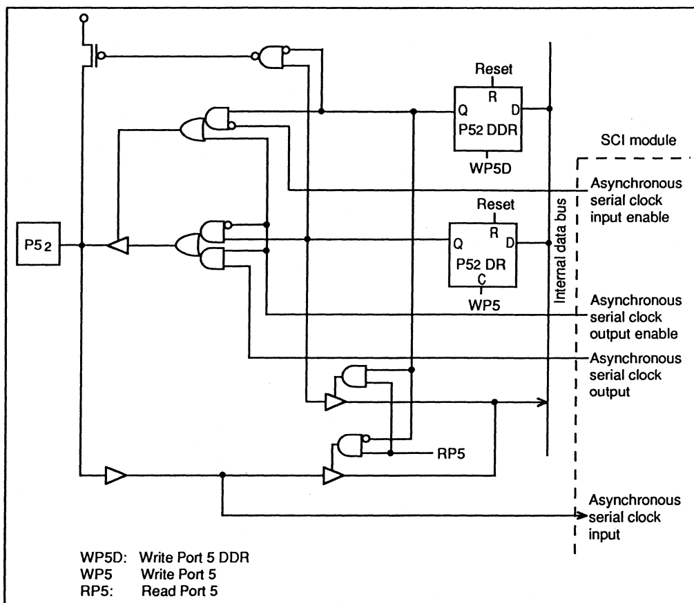
Figure 5-8. Port 5 Schematic Diagram (Pin P52)
