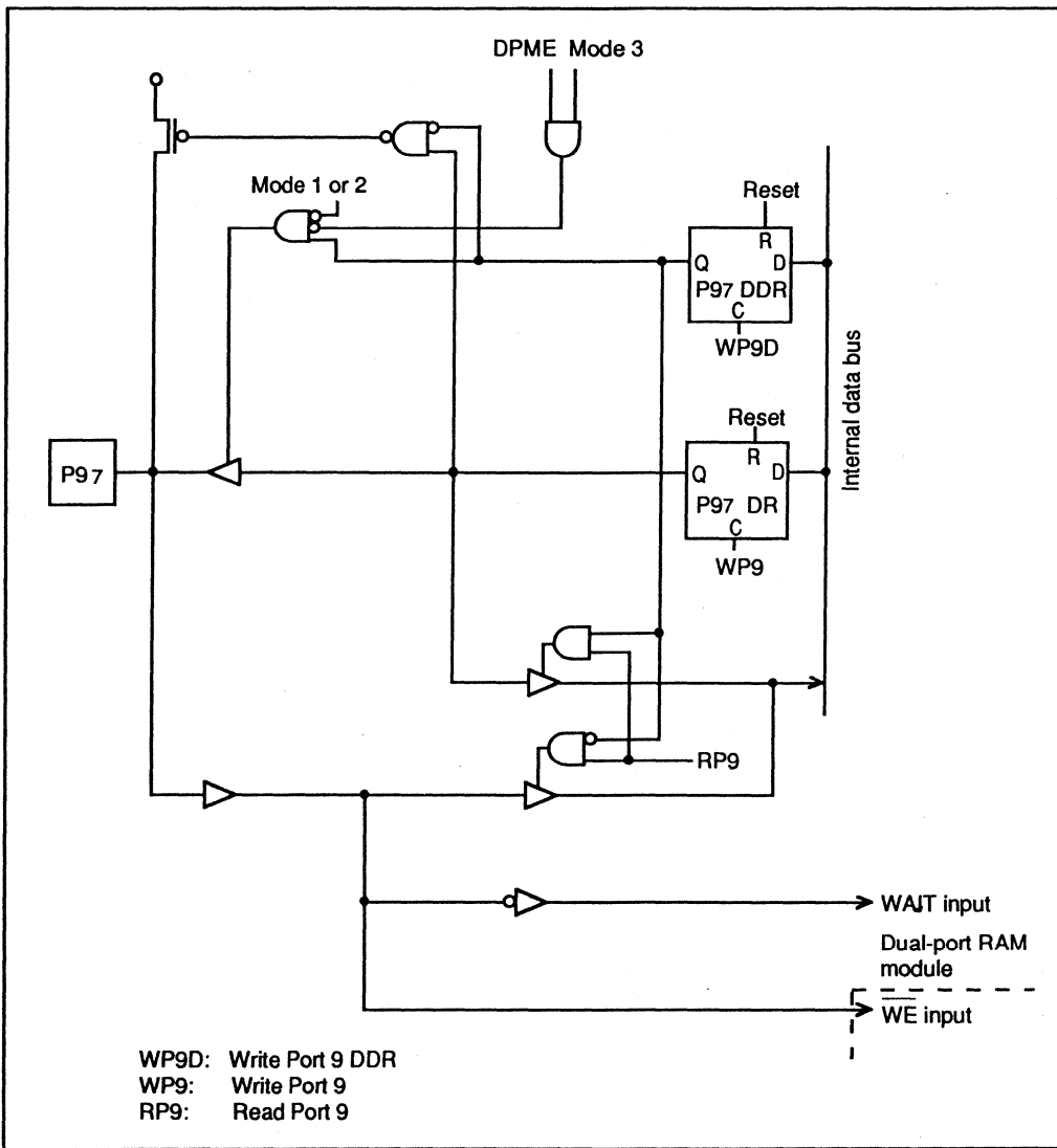
Figure 5-25. Port 9 Schematic Diagram (Pin P97)
