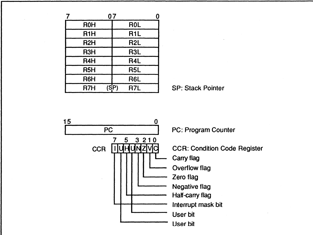
Figure 3-1. CPU Registers
