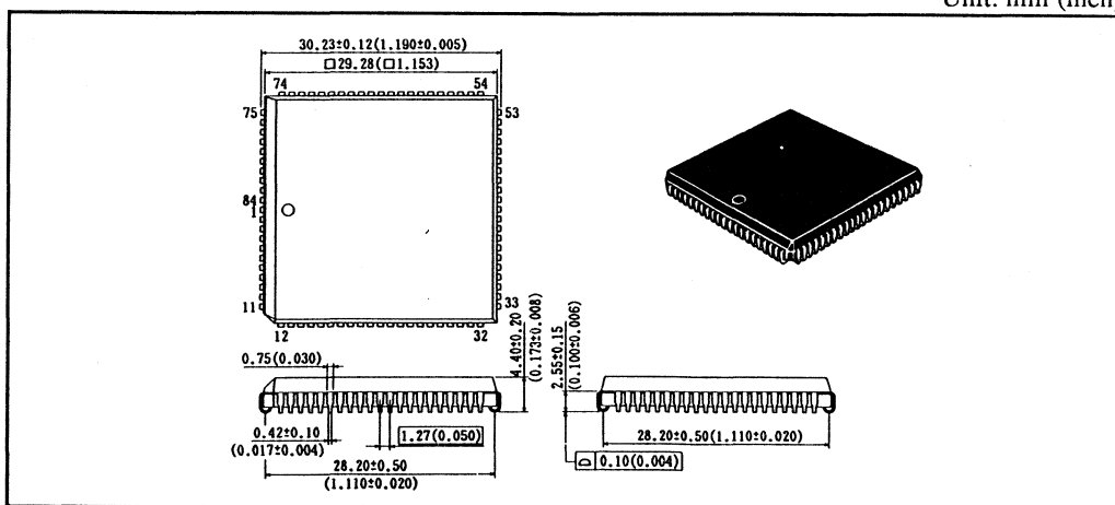
Figure D-2. Package Dimensions (CP-84)
