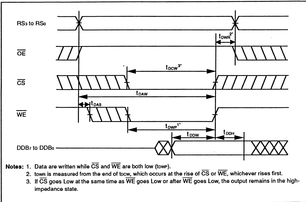
Figure 17-21. Dual-Port RAM Write Timing
