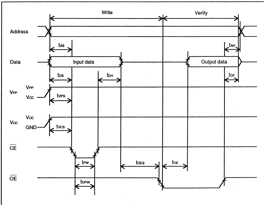
Figure 13-5. PROM Write/Verify Timing
