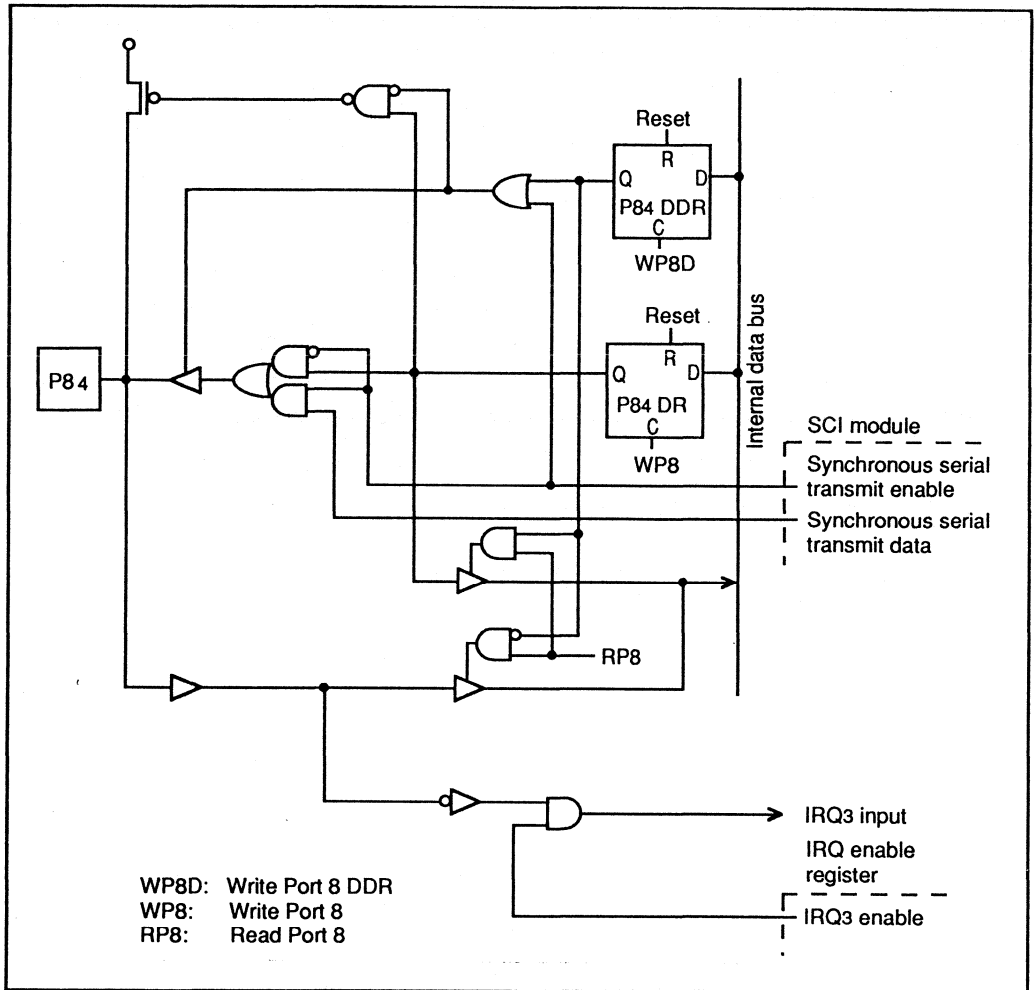
Figure 5-17. Port 8 Schematic Diagram (Pin P84)
