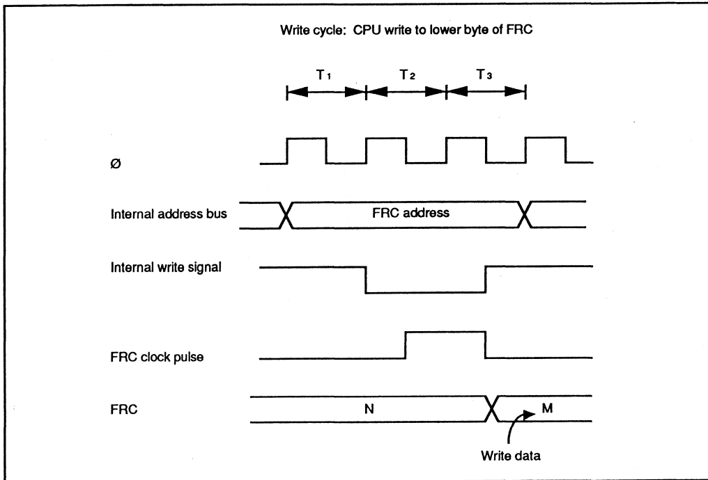
Figure 6-22. FRC Write-Increment Contention
