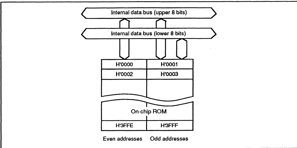
Figure 13-1. Block Diagram of On-Chip ROM
