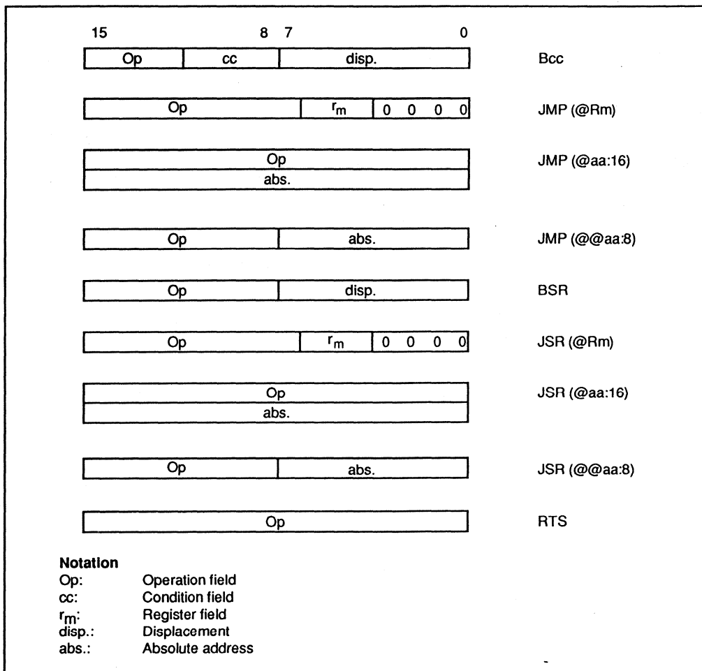
Figure 3-8. Branching Instruction Codes
