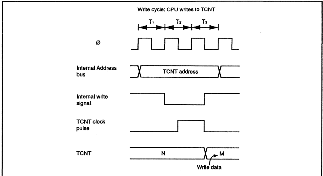
Figure 7-14. TCNT Write-Increment Contention
