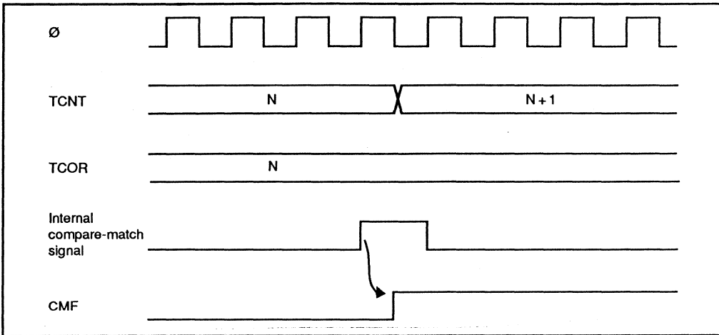
Figure 7-5. Setting of Compare-Match Flags
