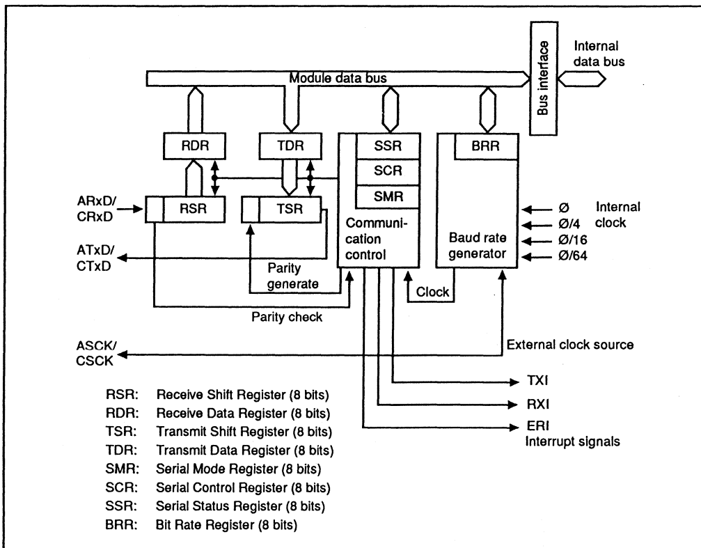
Figure 9-1. Block Diagram of Serial Communication Interface
