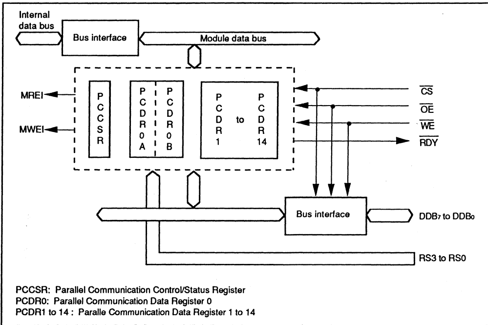
Figure 11-1. Block Diagram of Dual-Port RAM
