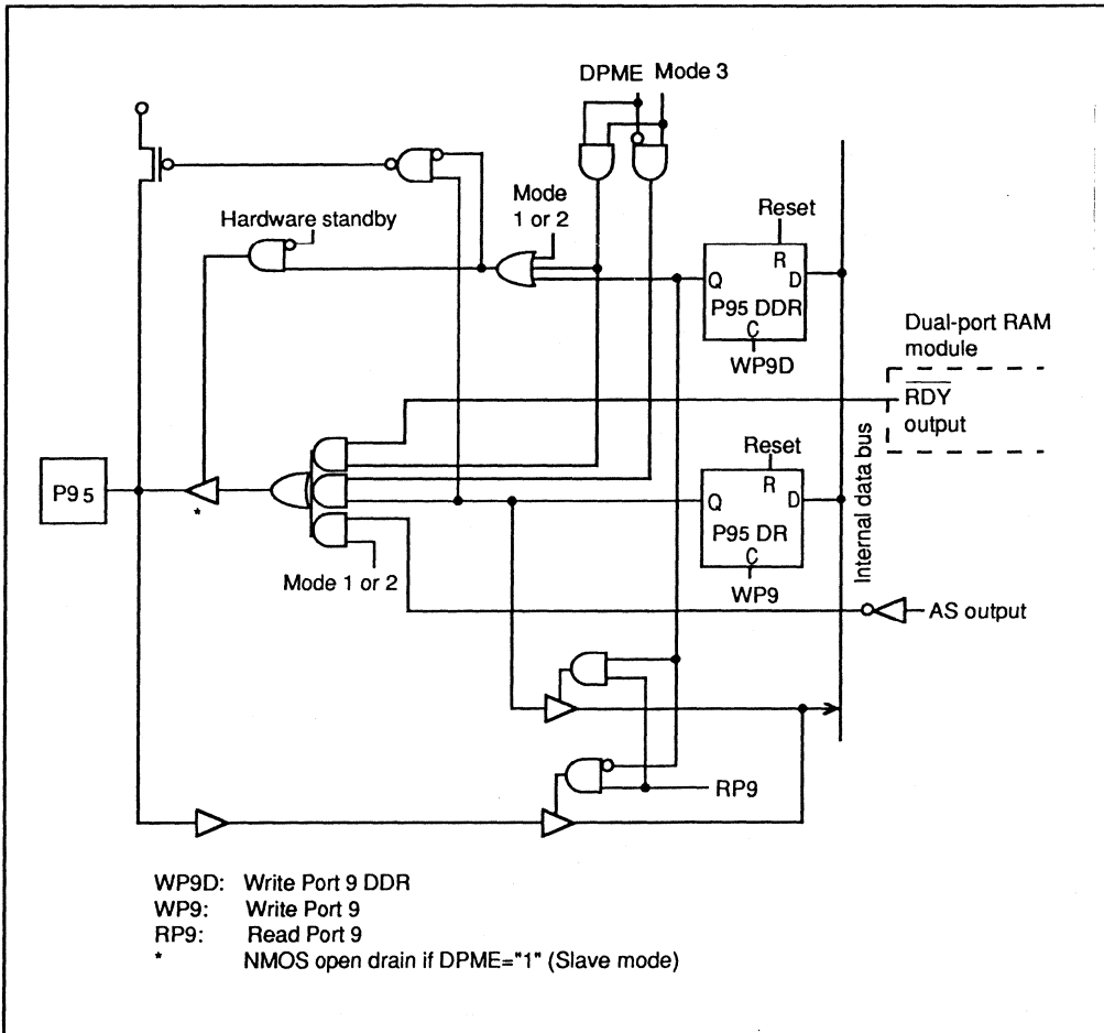
Figure 5-23. Port 9 Schematic Diagram (Pin P9s)
