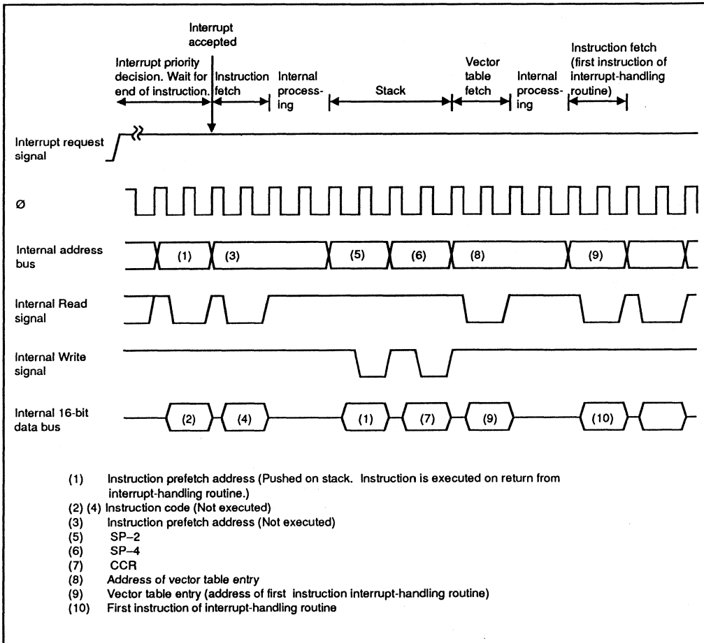
Figure 4-5. Timing of Interrupt Sequence
