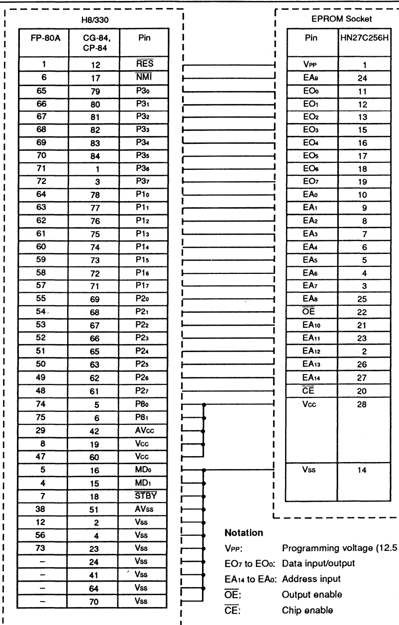
Figure 13-2. Socket Adapter Pin Assignments
