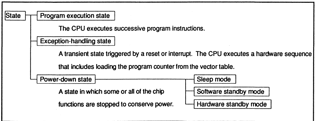
Figure 3-11. Operating States
