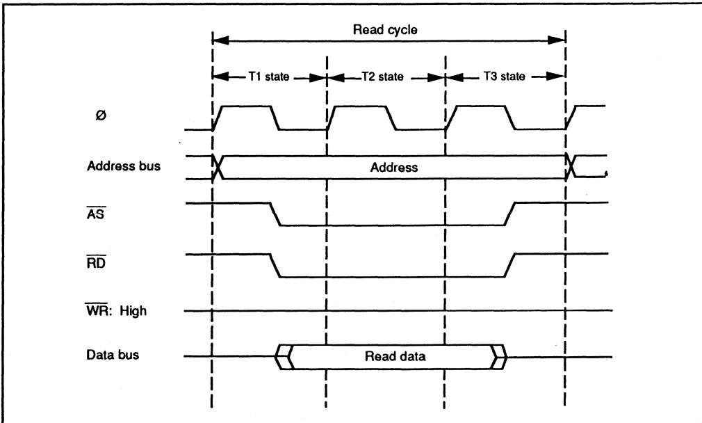
Figure 3-17 (a). External Device Access Timing (read)
