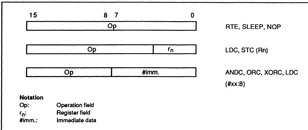
Figure 3-9. System Control Instruction Codes
