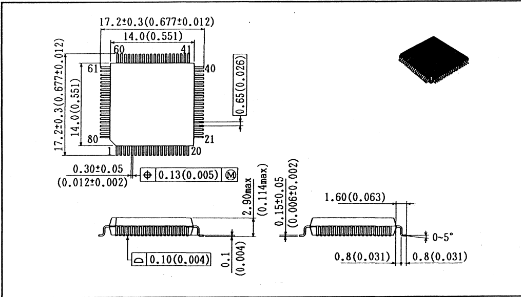
Figure D-3. Package Dimensions (FP-80A)
