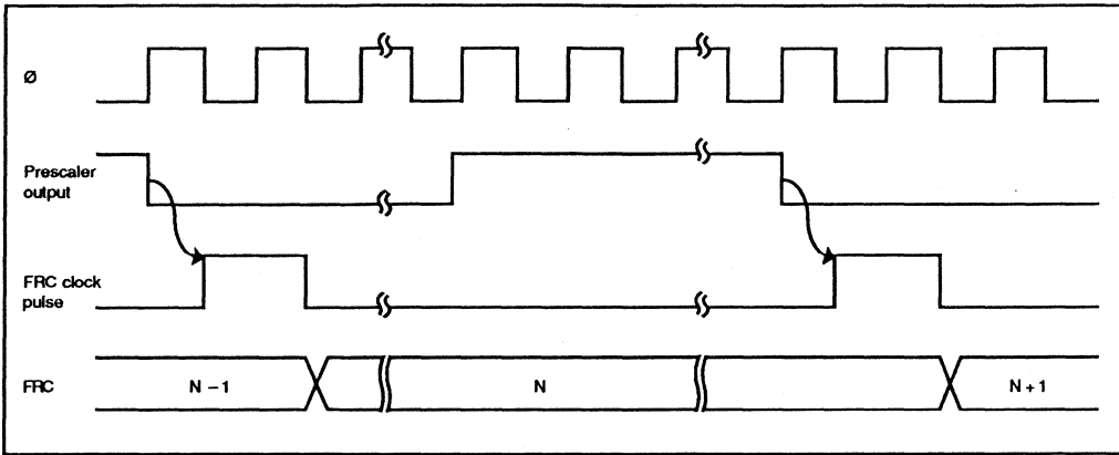
Figure 6-5. Increment Timing for Internal Clock Source
