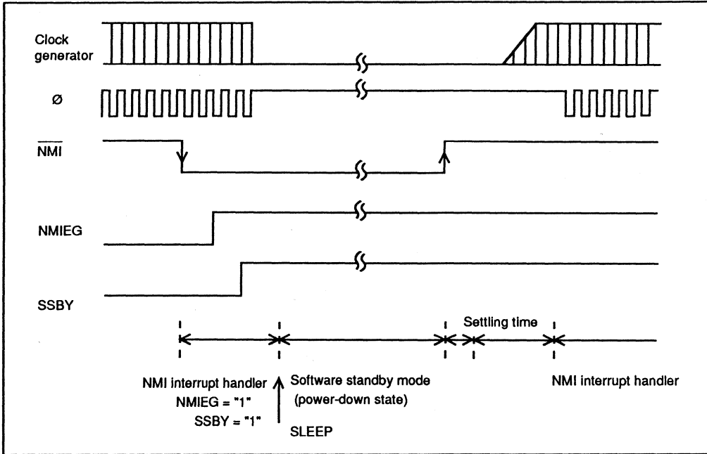
Figure 14-1. Software Standby Mode (when) NMI Timing
